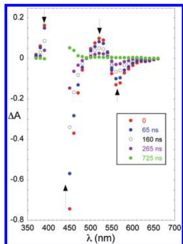
Figure 7. Transient spectra recorded when an O_2 saturated solution of [Co(TpivPP)(2-MeHIm)] ( [Co(TpivPP)] ( 3.59 \times 10^{-5} M) in 2.80 \times 10^{-3} M 2-MeHIm benzene solution) was irradiated at 351 nm. The delays from the laser flash are indicated in the figure.
