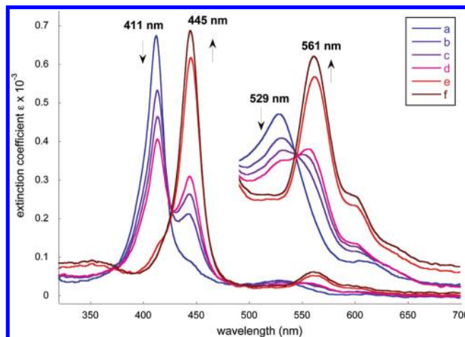
Figure 5. Selected UV-vis spectra taken in benzene. (a) [Co(II)(TpivPP)] ( 3.53 \times 10^{-5} M) in 1.22 \times 10^{-1} M 2-MeHIm solution. (b) The solution was exposed to air for 15 min. (c) The solution was exposed to air for 30 min. (d) The solution was exposed to air for 40 min. (e) The solution was exposed to air for 5 h. (f) The solution was exposed to air overnight.
