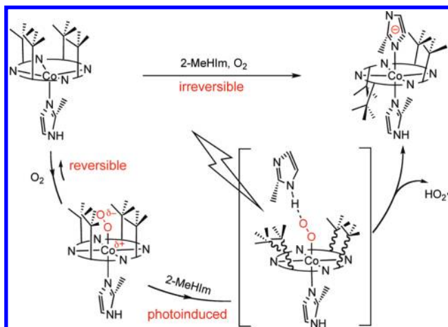
Scheme 1. Proposed Reaction Route to the Formation of [Co(III)(\alpha,\alpha,\beta\text{-TpivPP})(2-MeHIm)(2-MeIm^-)] from [Co(II)(TpivPP)(2-MeHIm)]
