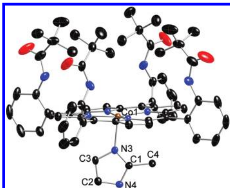
Figure 1. Thermal ellipsoid plot of [Co(II)(TpivPP)(2-MeHIm)] displaying a partial atom labeling scheme. The molecule has a required 2-fold axis of symmetry perpendicular to the porphyrin plane. Thus the axial imidazole is disordered over two positions related by the required symmetry axis, but only one orientation is shown. Thermal ellipsoids of all atoms are contoured at the 50% probability level. Hydrogen atoms have been omitted for clarity.
