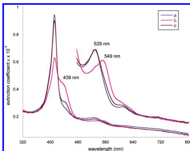
Figure 6. Selected UV-vis spectra taken in benzene. The spectra from 480 to 800 nm are measured in the 10 mm UV cell. (a) [Co(II)(TpivPP)] ( 3.59 \times 10^{-5} M) in 5.97 \times 10^{-3} M 2-MeHIm solution. (b) Oxygen bubbled for 3 min. (c) Argon purge for 5 min.
