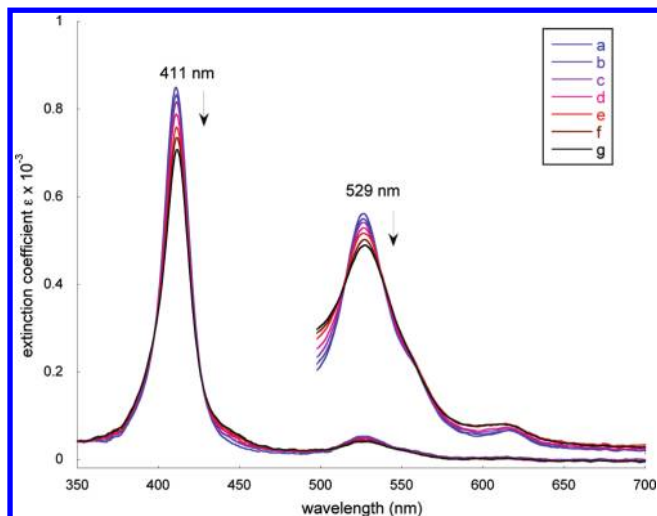
Figure 4. Selected UV-vis spectra taken in benzene under argon. The enlarged spectra from 500 to 700 nm are measured in the 10 mm UV cell. (a) [Co(II)(TpivPP)] ( 3.59 \times 10^{-5} M). (b) [Co(II)(TpivPP)] in 2.40 \times 10^{-5} M 2-MeHIm solution. (c) [Co(II)(TpivPP)] in 6.00 \times 10^{-3} M 2-MeHIm solution. (d) [Co(II)(TpivPP)] in 1.20 \times 10^{-4} M 2-MeHIm solution. (e) [Co(II)(TpivPP)] in 2.40 \times 10^{-4} M 2-MeHIm solution. (f) [Co(II)(TpivPP)] in 4.76 \times 10^{-4} M 2-MeHIm solution. (g) [Co(II)(TpivPP)] in 1.06 \times 10^{-3} M 2-MeHIm solution.
