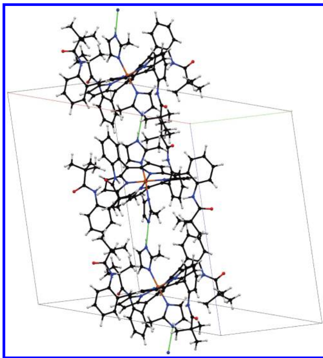
Figure 3. Partial packing diagram of complex [Co(TpivPP)(2-MeHIm)(2-MeIm − )](monoclinic) showing the unit cell and the hydrogen bonds between the axial ligands. A second chain of opposite helicity exists in the complete crystal structure.
